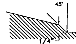
LIP DETAIL
